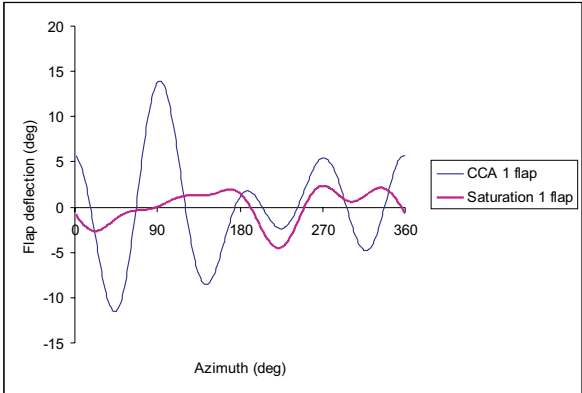
Figure 16: Flap deflections, effect of saturation, \mu=0.35 .
