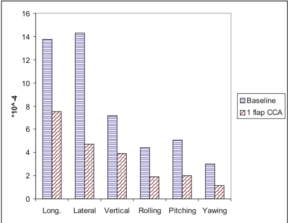
Figure 17: Vibration reduction, CCA, pretwist, \mu=0.35 .
