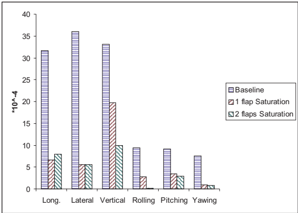
Figure 15: Vibration reduction with saturation limits, \mu=0.35 .
