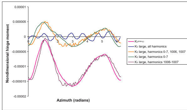
Figure 10: Flap hinge moment for prescribed flap deflections ( K_\delta = +\infty ) and for a large value of K_\delta ; \delta_a=0 ; and \mu=0.35 .
