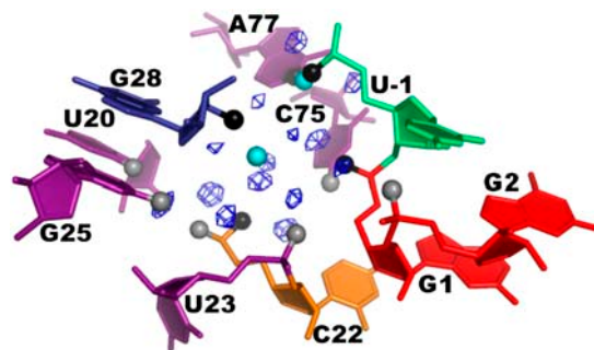
FIGURE 5 Two Na + cations (cyan balls) and their hydration shell (blue mesh) bound at the catalytic pocket in simulation PreC41+A-2. Positions of cations in the figure are determined by points with highest pseudo-electron density of Na + . The residues are color-coded as in Fig. 1; functional groups of the catalytic pocket directly bound to the Na + are shown as black balls and those interacting with the first hydration shell waters as gray balls.
