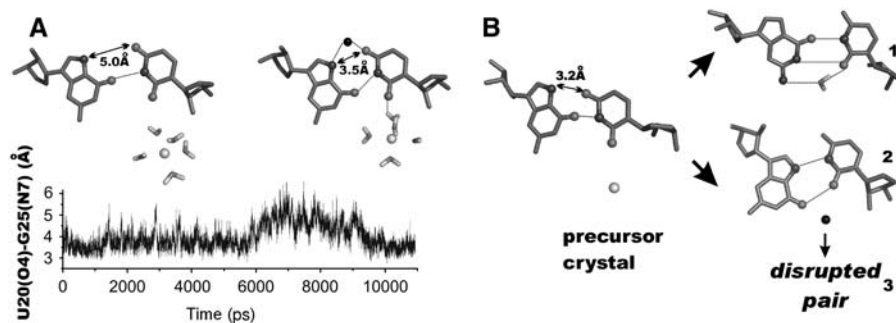
FIGURE 4 Interactions of the U20/G25 basepair with cations in precursor simulations. Basepair edge oriented inside the catalytic pocket is directed downward. Gray and black balls represent Mg^{2+} and Na^+ cations, respectively. (A) Two substates seen in precursor simulations with Mg^{2+} . The U20(O4)-G25(N7) distance trajectory in simulation PreC41+A-2 is shown below. (B) Rearrangement of the U20/G25 basepair in the absence of Mg^{2+} ; arrows show transitions observed in simulations. Substates 1–3 were observed in the following simulations: 1), PreC41+ and PreC41+A-2; 2), PreC41+C75+, PreC41+U75, PreC41+A-2 and PreC41+U75A-2; and 3), PreC41+Trc and PreC41+U75.
