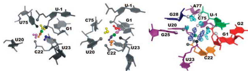
FIGURE 3 First hydration shell of \text{Mg}^{2+} bound at the catalytic pocket in simulations PreC41+U75A-2Mg (left) and PreC41+A-2Mg before the G1(O5')... \text{Mg}^{2+} water bridge was broken (middle). (Right) First and second hydration shells of the catalytic \text{Mg}^{2+} in the simulation PreC41+A-2Mg (after the G1(O5')... \text{Mg}^{2+} water bridge was lost). The residues are color-coded as shown in Fig. 1. \text{Mg}^{2+} is represented by a green ball; dark blue and cyan mesh represent first and second hydration shells of \text{Mg}^{2+} ,
