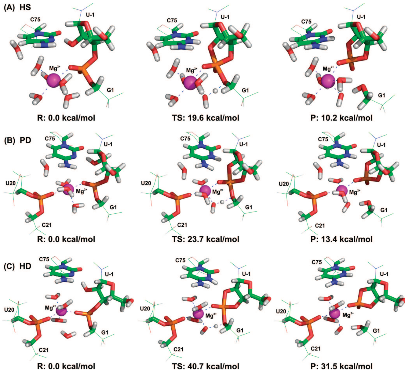
Figure 4. Structures of HDV ribozyme active sites and the corresponding MPW1K/6-31+G(d,p):AMBER(parm99) energies in precursor (R), transition (TS), and product (P) states of the following reaction profiles with different Mg 2+ ion positions and coordinations: (A) the structure including a hexacoordinated Mg 2+ ion with a single inner-shell bond to the G1(O1P) oxygen of the scissile phosphate (denoted HS in the text), (B) the structure including a pentacoordinated Mg 2+ ion with double inner-shell contacts to phosphates from C21 and G1 (denoted PD), and (C) the structure including a hexacoordinated Mg 2+ ion with double inner-shell bonds to phosphates from C21 and G1 (denoted HD). The quantum region and part of the molecular mechanical model neighborhood are shown in sticks and wire representation, respectively.
