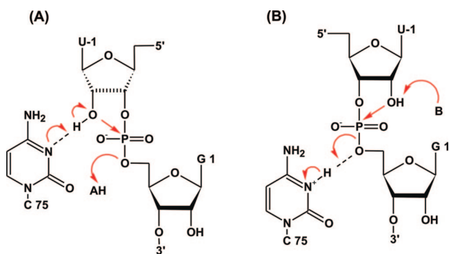
Figure 2. Two proposed general acid–base reaction mechanisms for HDV ribozyme: (A) C75 general base mechanism; the U-1(O'2) nucleophile is deprotonated by nucleobase C75 acting as a general base. The leaving G1(O'5) alcoholate group is protonated by a general acid (e.g., a water molecule coordinated to the Mg^{2+} ion). (B) General acid mechanism; the leaving G1(O'5) alcoholate group is protonated by nucleobase C75 acting as a general acid and the (U-1)O'2 nucleophile is deprotonated by a general base.
