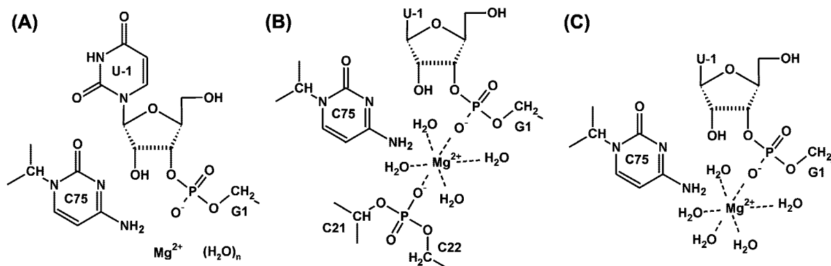
Figure 3. Schemes of three quantum regions used in QM/MM calculations. (A) The large quantum region was used for a rapid preoptimization of the HDV ribozyme active site with an Mg^{2+} ion in 13 different positions. The number of water molecules ranged from 13 to 25 depending on the position of the Mg^{2+} ion. (B) The quantum region used to study the reaction energy profile for reaction coordinates including the Mg^{2+} ion with double inner-shell arrangements (PD and HD structures). (C) The quantum region used to study the reaction energy profile for the reaction coordinate including the Mg^{2+} ion with single inner-shell arrangement (HS).
