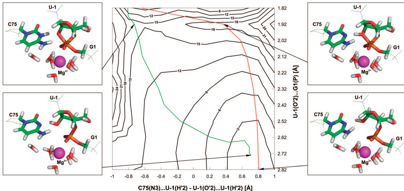
Figure 5. Two-dimensional map of the potential energy surface (More O'Ferrall-Jencks diagram). The energy is presented as a function of the distance between U-1(O'2) and G1(P) (vertical axis) and the difference between two U-1(H'2)-C75(N3) and U-1(O'2)-H'2 distances describing the proton transfer. The energy (kcal/mol) was calculated by the BLYP/cc-pVDZ:AMBER(parm99) method. The red line describes the reaction coordinate obtained by shortening the U-1(O'2)-G1(P) distance following the reaction from precursor to product, while the green line presents the reaction coordinate obtained by scanning the backward reaction from products to precursor via shortening the G1(O'5)-P distance (see text for details). The structures related to the corresponding parts of the surface are shown in small boxes.
