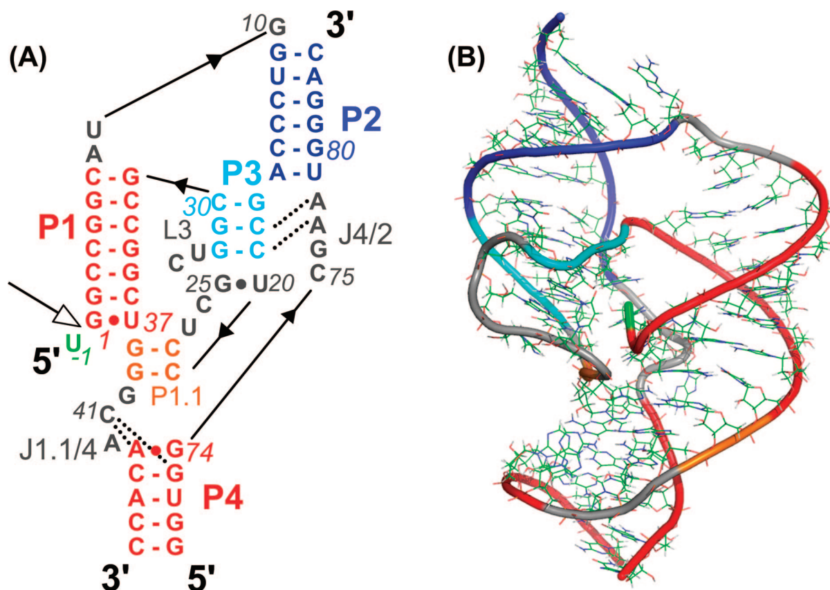
Figure 1. Structure of the precursor form of HDV ribozyme: (A) Sequence and secondary structure of the HDV ribozyme genomic form. The scissile phosphate between U-1 and G1 is highlighted by an open arrow (panel taken from ref 13 ). (B) Three-dimensional structures of the HDV ribozyme. The colors of the structural elements correspond to those in A.
