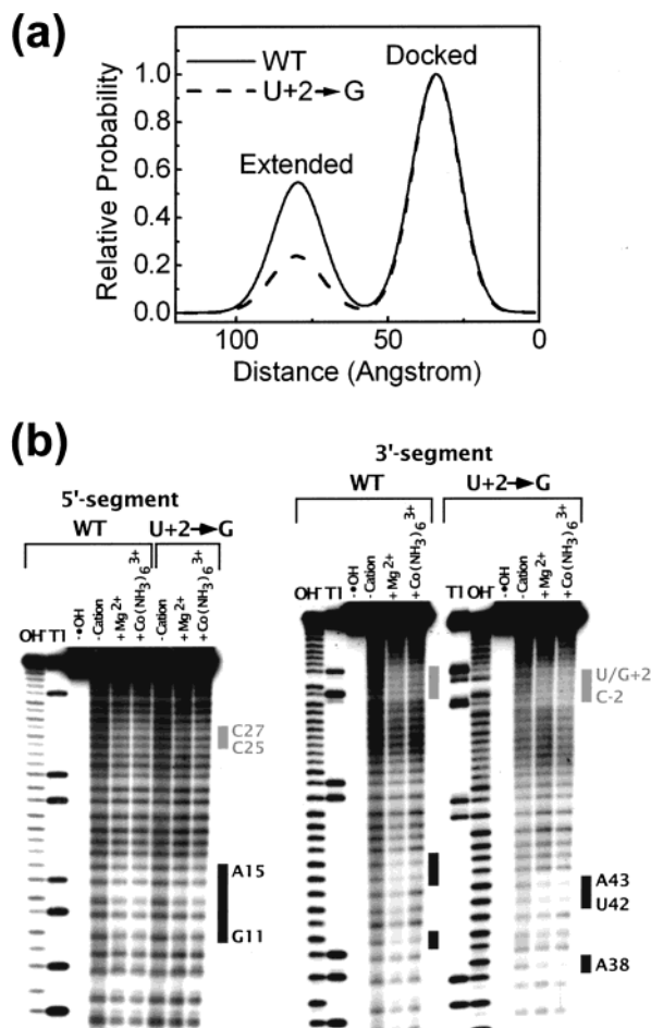
FIGURE 3: Comparison of the docked conformers of the wild-type (WT) and U+2f G mutant hairpin ribozyme-substrate complexes. (a) Normalized donor-acceptor distance distributions for the WT (solid line) and mutant (dashed line) ribozyme-substrate complexes as measured by trFRET in standard buffer at 17.8 °C (see Materials and Methods) (10). While the distance distributions of the extended (mean distance: 78 \pm 1 Å) and docked (mean distance: 34 \pm 1 Å) conformers are indistinguishable, the relative abundance of docked complex increases from 65 \pm 1\% to 81 \pm 1\% upon introducing the U+2f G mutation, equivalent to 0.5 kcal/mol additional stabilization energy. (b) Solvent-protected core of WT and U+2f G mutant ribozyme-substrate complexes as observed by hydroxyl-radical footprinting (see Materials and Methods) (9). Both the 5'- and 3'-segments of the two-strand WT and U+2f G mutant ribozyme-substrate complexes were analyzed in the absence (-) and presence (+) of 12 mM Mg^{2+} and 1.5 mM Co(NH_3)_6^{3+} , as indicated, together with a control without hydroxyl radicals (-OH). Partial hydrolysis with alkali (OH - ) and ribonuclease T1 (shifted up by one nucleotide compared to the hydroxyl radical pattern) (9) served to identify protected areas, highlighted in the same shades as in Figure 1(a).
