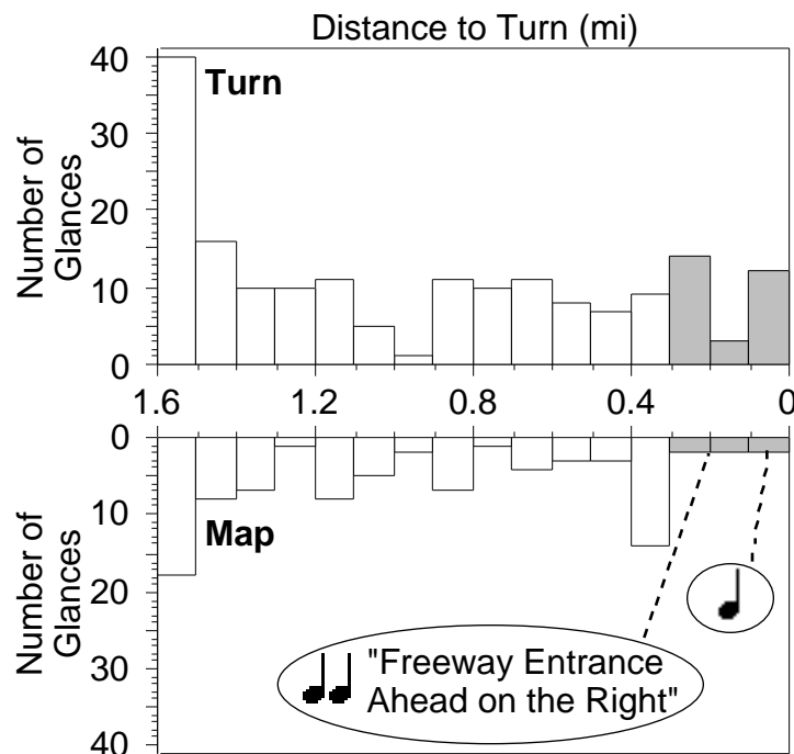
Figure 14. Distance to turn for medium (1.5-mile) city road segment.
