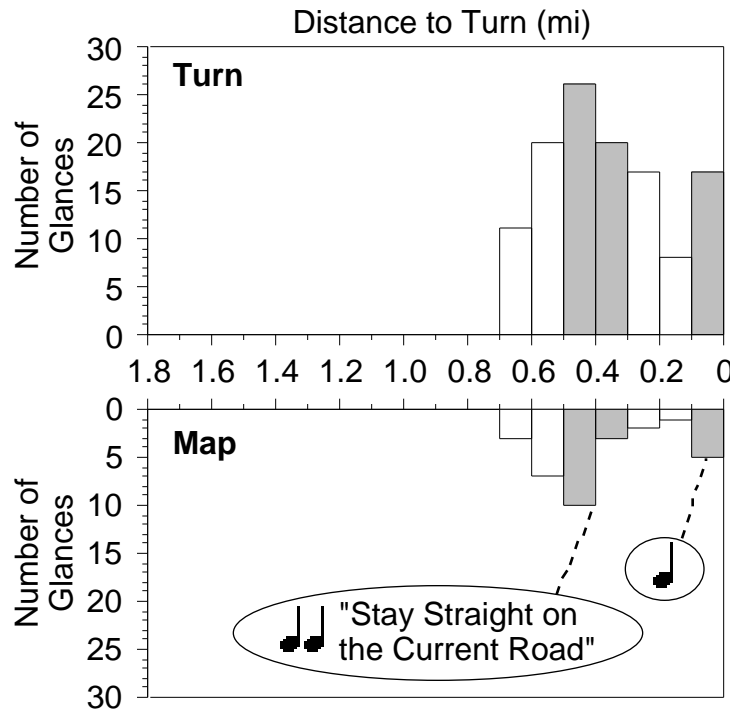
Figure 10. Distance to turn for short (0.6-mile) freeway segment.
