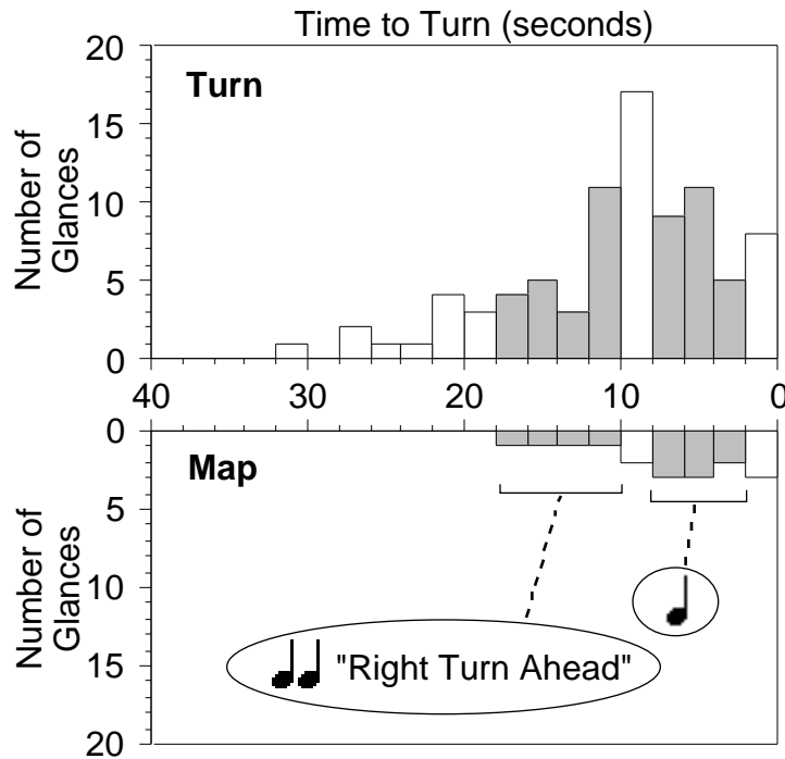
Time to turn for two short (0.0-mile) city road segments.
