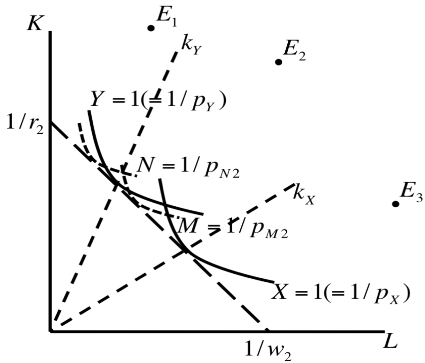
Figure 1: Autarky Equilibria
