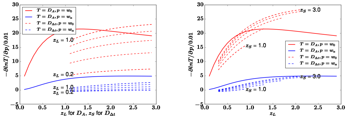
Figure 2. Logarithmic derivatives of distances T = (D_A, D_{\Delta t}) with respect to the cosmological parameters p = (w_0, w_a) , as a function of redshift. Left panel: the solid lines show T = D_A , while the dashed lines show T = D_{\Delta t} , with various combinations of the lens and the source redshift. Each dashed line corresponds to one z_L in range [0.2, 1.0] in increments of 0.2, and shows -\partial \ln D_{\Delta t} / \partial p / 0.01 as a function of z_S . We only show z_S which is higher than the highest z_L in this range. Right panel: the solid lines show -\partial \ln D_A / \partial p / 0.01 as a function of z_L . Each dashed line corresponds to one z_S in range [1.0, 3.0] in increments of 0.5, and shows -\partial \ln D_{\Delta t} / \partial p / 0.01 as a function of z_L . We only show z_L which is lower than the lowest z_S in this range. Both panels show that D_A is always more informative than D_{\Delta t} for constraining w_a (i.e., |\partial \ln D_A / \partial w_a| > |\partial \ln D_{\Delta t} / \partial w_a| ), and D_A is often more informative than D_{\Delta t} on w_0 .
