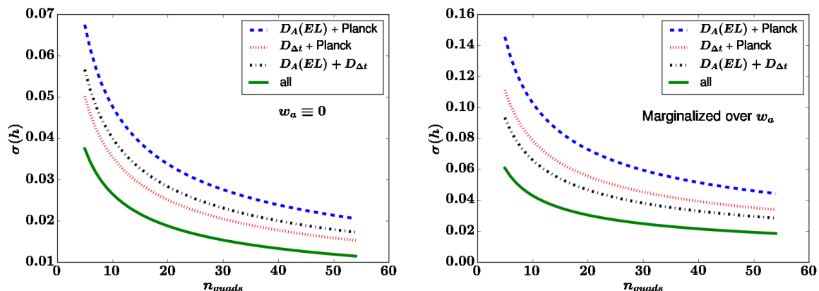
Figure 9. The 1\text{-}\sigma uncertainty in h = H_0/100 km/s/Mpc from time-delay lenses as a function of the number of quadruply imaged lenses for the (left) ow CDM model, and (right) ow_z CDM model.
