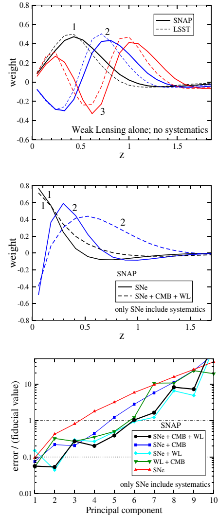
FIG. 1 (color online). Top : three best-measured principal components of w(z) for the upcoming weak lensing surveys; higher depth and galaxy density (SNAP) and wider area (LSST) each contribute well. Note that the best-measured mode peaks at z \sim 0.4 . Middle : Two of the best-measured PCs of w(z) expected for a SNAP-type survey for SN alone, and SN combined with weak lensing and CMB (Planck d_A(z_{\text{Iss}}) ). The best PC from SN alone peaks at z \sim 0 ; this becomes z \sim 0.2 , if \Omega_M is independently known to better than 0.01 (not shown). Note that the second best-measured PC is pushed out to higher redshift once the WL and CMB information is added in. Bottom : Inverse signal-to-noise in measuring the PCs of w(z) ; that is, accuracies in measuring the PC coefficients divided by their fiducial values. We show the cases of SN alone, SN + CMB, SN + WL, WL + CMB, and the three probes combined. Throughout, we include the systematics in SN constraints, but not in WL estimates as the systematics contributions to the latter are highly uncertain.
