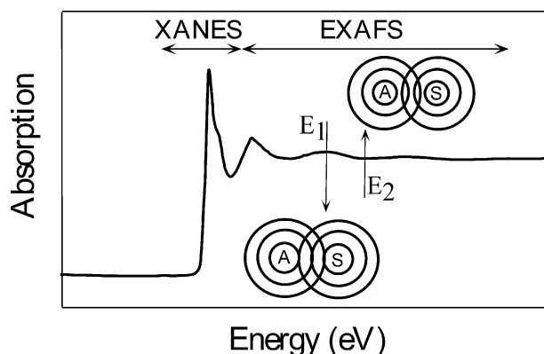
Fig. 1. Schematic illustration of an X-ray absorption spectrum at the Zn K-edge. The insets show the interference phenomena that give rise to the modulations in absorption cross-section (see text). In the insets, A and S refer to the absorbing and scattering atoms, respectively. The concentric circles around A and S represent the maxima in the photoelectron wave that describes the propagation of the X-ray excited photoelectron. Constructive interference between the outgoing and back-scattered waves ( E_1 ) give a local maximum in absorption; destructive interference ( E_2 ) gives a local minimum.
