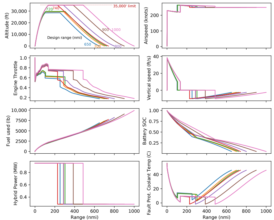
Figure 16. Optimized flight profile and control parameters—various ranges.
