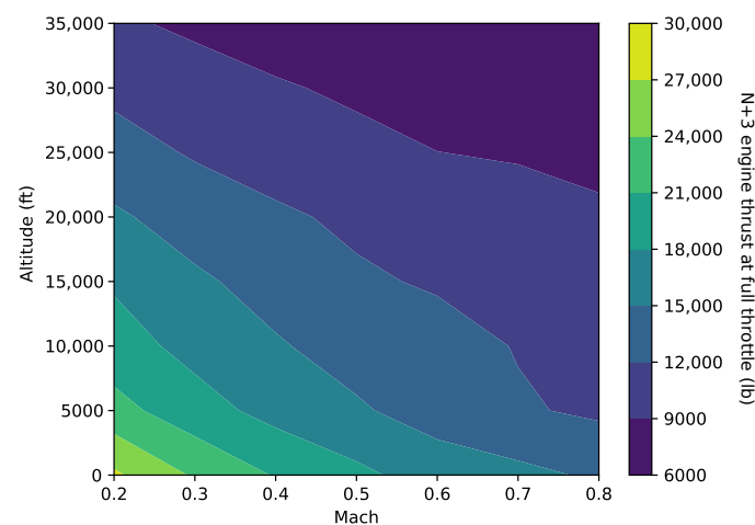
Figure 2. The maximum thrust of the N+3 engine decreases quickly with increasing speed and altitude. The maximum thrust values are constrained by spool shaft speed and turbine inlet temperature limits.
