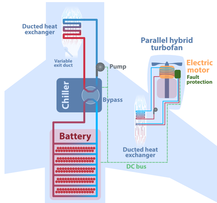
Figure 5. The VCS thermal management system actively cools the battery with an electrically-powered vapor cycle chiller and passively cools the electric motor and its fault protection.
