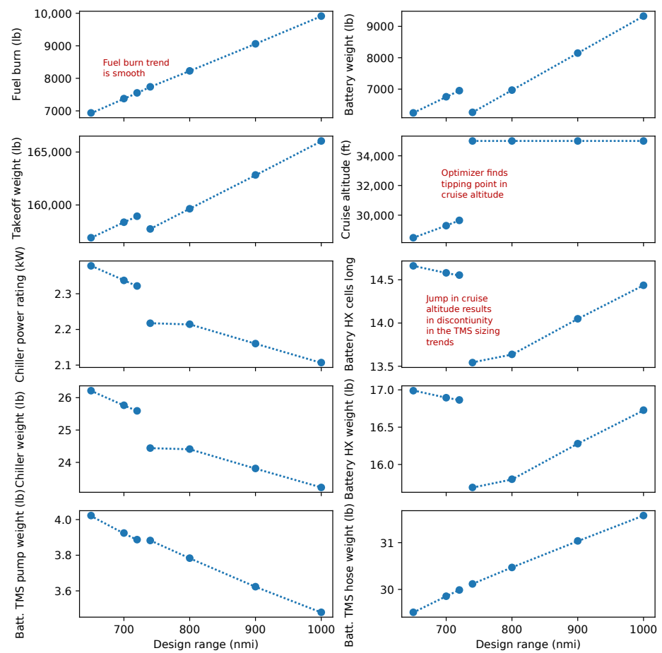
Figure 15. Effect of mission range on optimal design.
