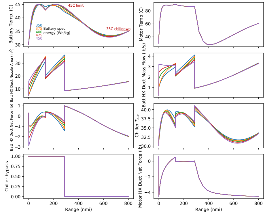
Figure 22. Optimized thermal trajectory and control parameters for various battery-specific energies (800 nmi flight).
