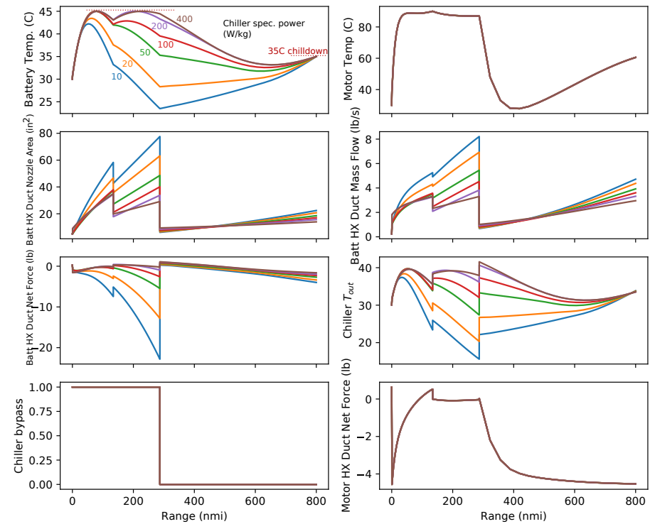
Figure 19. Optimized thermal trajectory and control parameters for various chiller-specific powers, with chillover.
