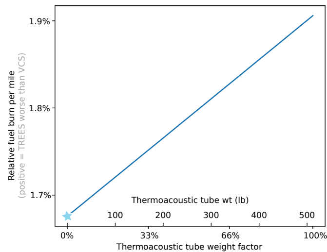
Figure 10. Increasing thermoacoustic tube weight from the baseline of 0 lbs to the full weight of the tubes results in over a 0.2% increase in fuel burn.
