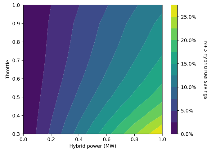
Figure 4. Compared to the fuel burn with electrical power off shown in Figure 3, adding electric power to the parallel hybrid N+3 engine’s electric motor reduces fuel burn by up to 25%. The flight condition in this plot is cruise at M = 0.8 and 35,000 ft.
