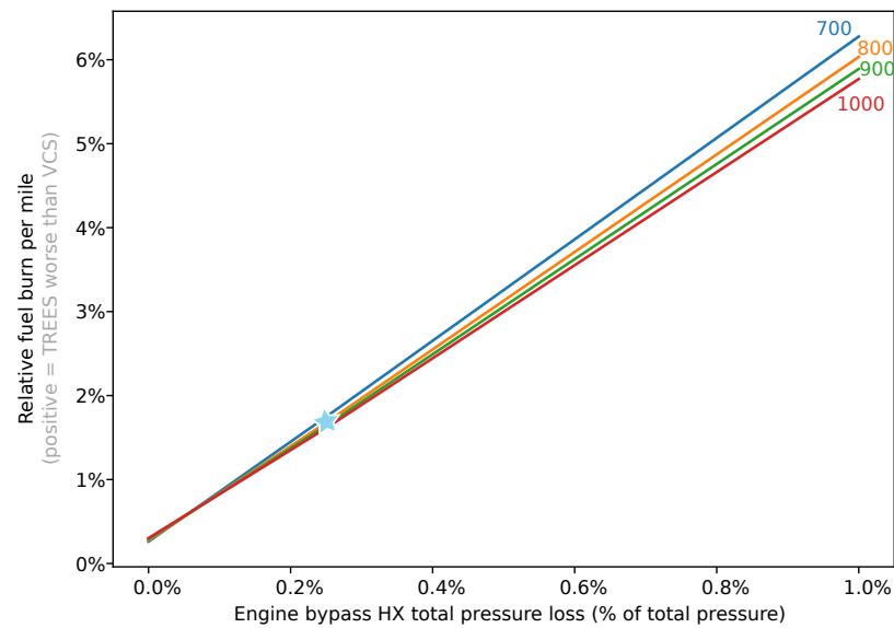
Figure 9. The bypass heat exchanger’s total pressure loss is by far the most significant technology parameter in determining the effectiveness of TREES. For these studies, we assume a baseline total pressure loss of 0.25%, marked by the blue star.
