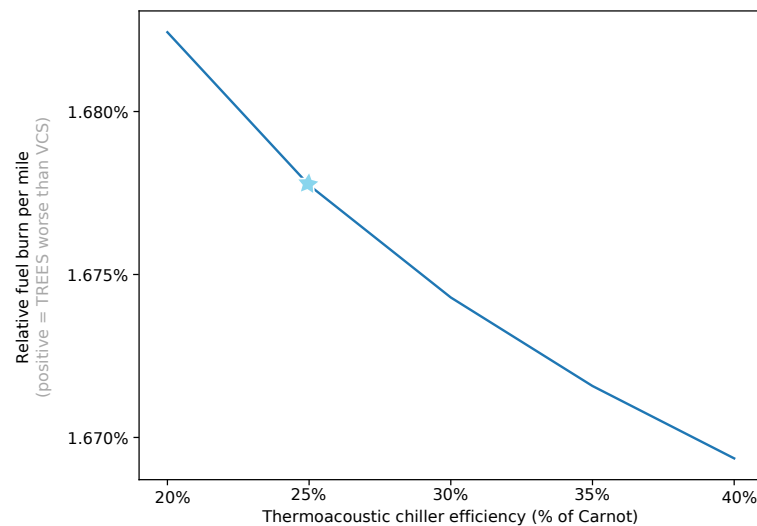
Figure 12. Higher thermoacoustic chiller efficiencies can pump more heat from the battery to the duct, which generates more thrust in the duct, saving fuel. The blue star marks the baseline chiller efficiency of 25%.
