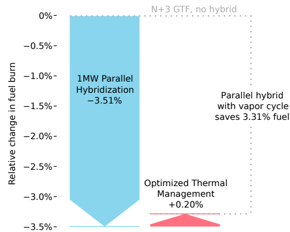
Figure 7. Relative to the conventional N+3 configuration with a geared turbofan, the parallel hybrid system with a vapor cycle chiller saves 3.31% fuel burn on an 800 nmi mission with 400 Wh/kg batteries.
