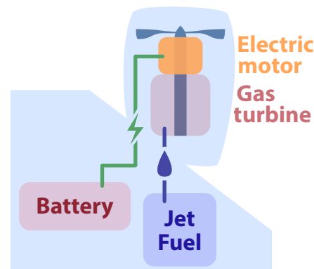
Figure 1. Parallel hybrid propulsion architecture.
