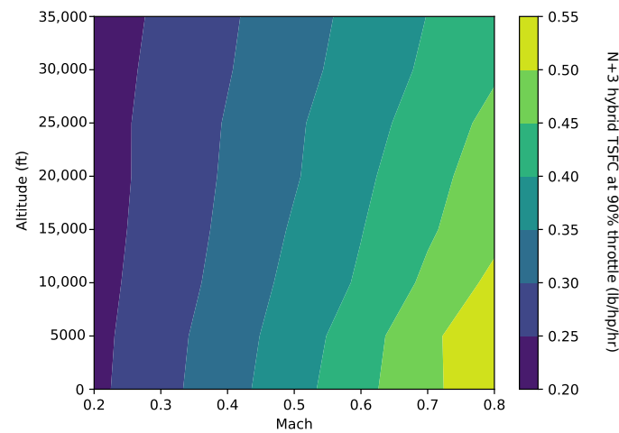
Figure 3. Thrust-specific fuel consumption of the optimized parallel hybrid N+3 at cruise throttle (90%) and zero electrical power input to the electric motor.
