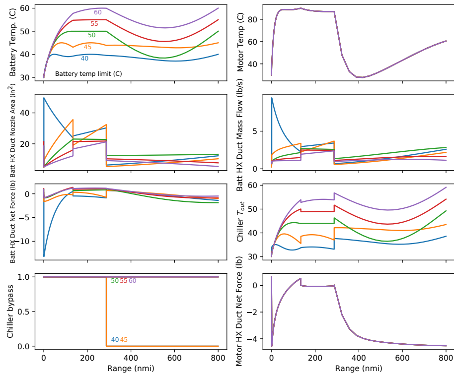
Figure 25. Optimized thermal trajectory and control parameters for various battery temperature limits.
