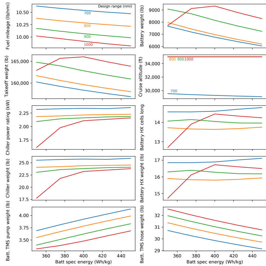
Figure 21. Effect of battery-specific energy on optimal design for various design ranges.
