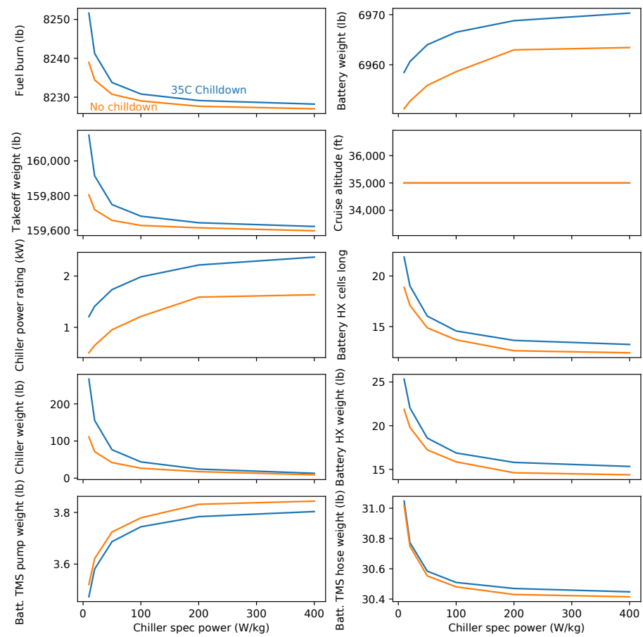
Figure 18. Effect of chiller-specific energy on optimal design.
