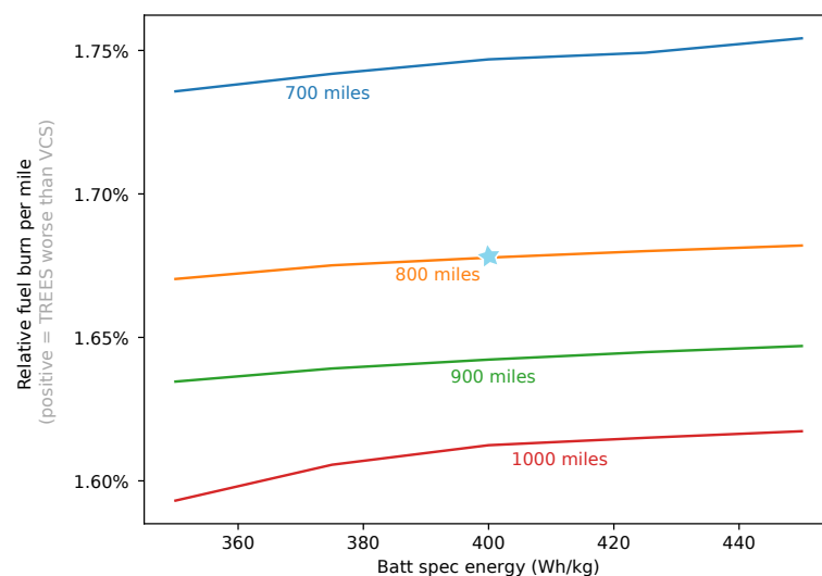
Figure 11. The vapor cycle chiller needs to carry batteries to power it, whereas TREES does not. This results in better relative performance for TREES on longer missions and with lower battery-specific energies than on shorter missions and with higher battery-specific energies. The blue star identifies the baseline mission.
