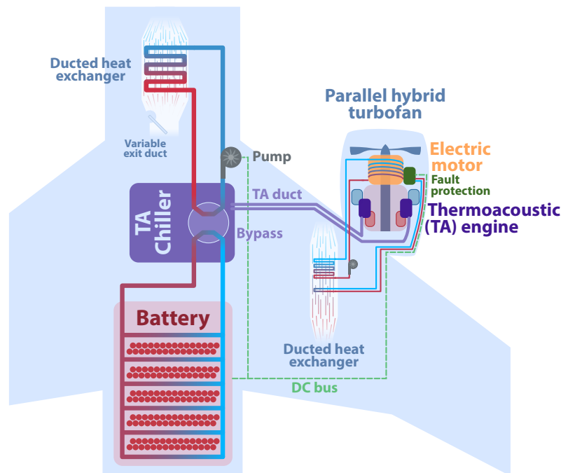
Figure 6. Thermal management system with TREES thermoacoustic chiller.
