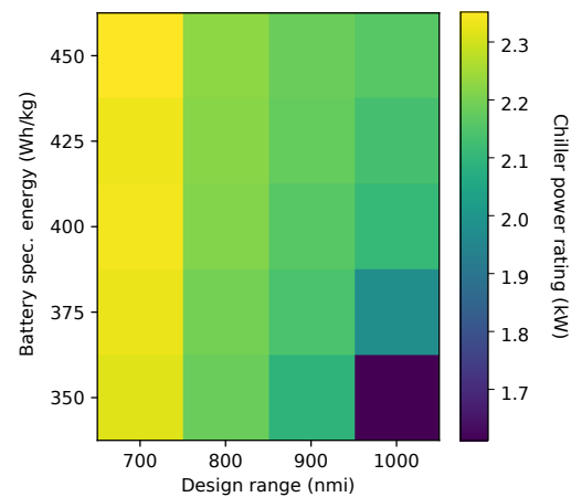
Figure 23. Optimal chiller size variation with flight length and battery-specific energy.
