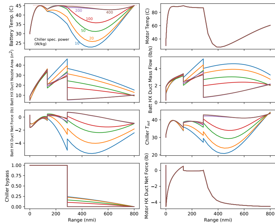
Figure 20. Optimized thermal trajectory and control parameters for various chiller-specific powers, without chilldown.
