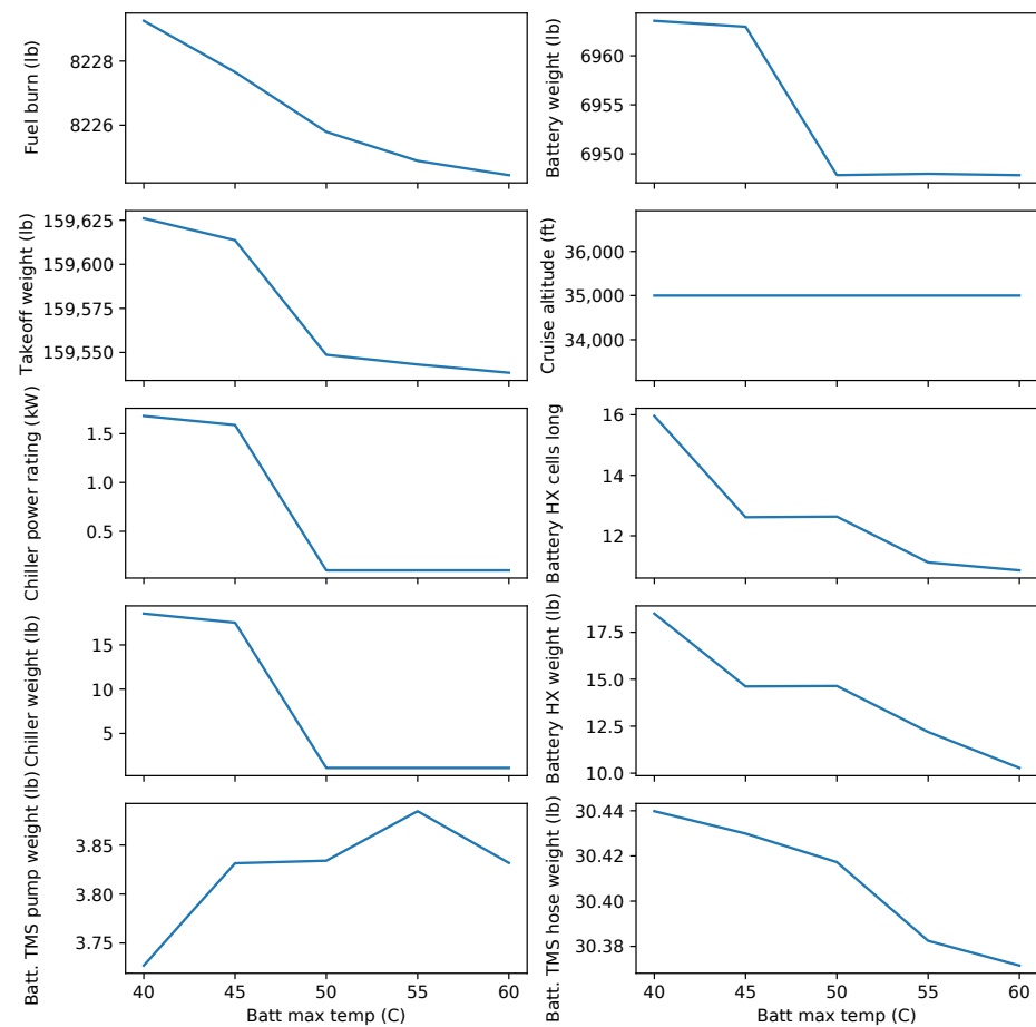
Figure 24. Effect of battery temperature limit on optimal design (800 nmi flight).
