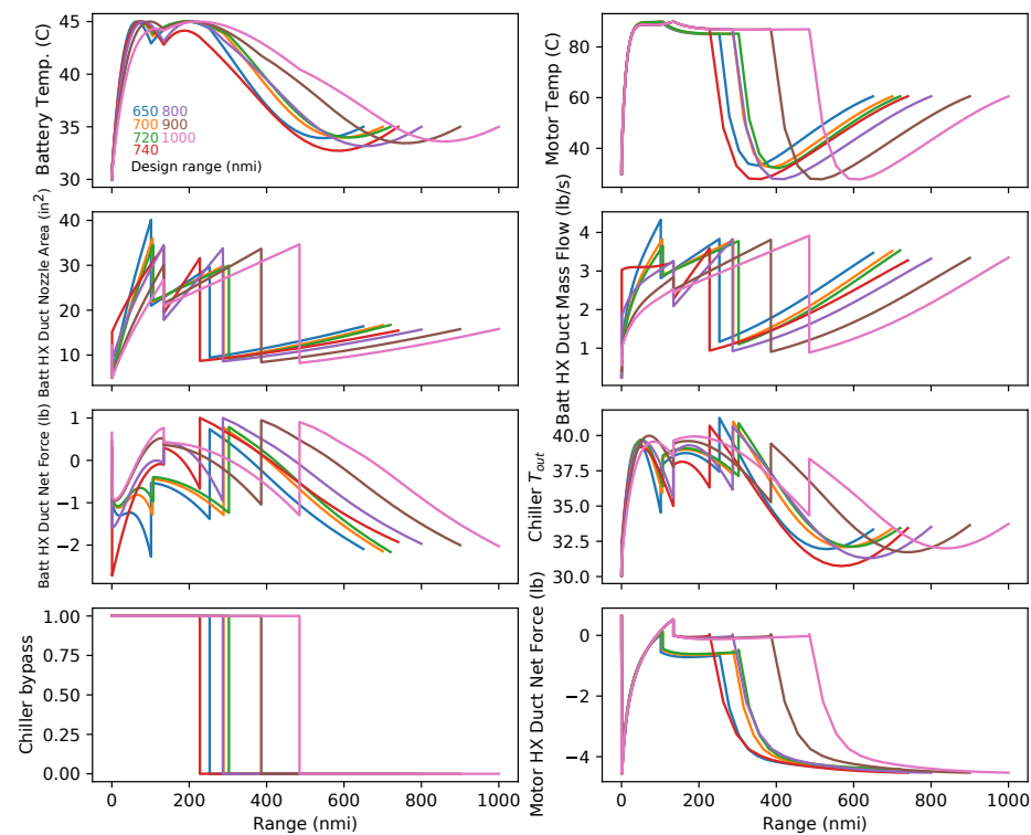
Figure 17. Optimized thermal trajectory and control parameters for various ranges.
