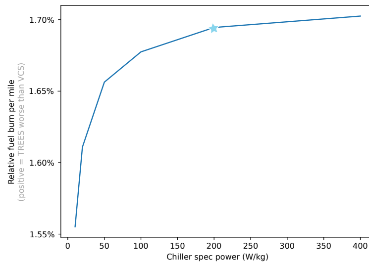
Figure 13. Varying vapor cycle chiller-specific power, we recover the expected fuel burn trend of decreasing fuel burn for the vapor cycle system aircraft that tapers off as specific power increases. The blue star shows the baseline specific power of 200 W/kg.
