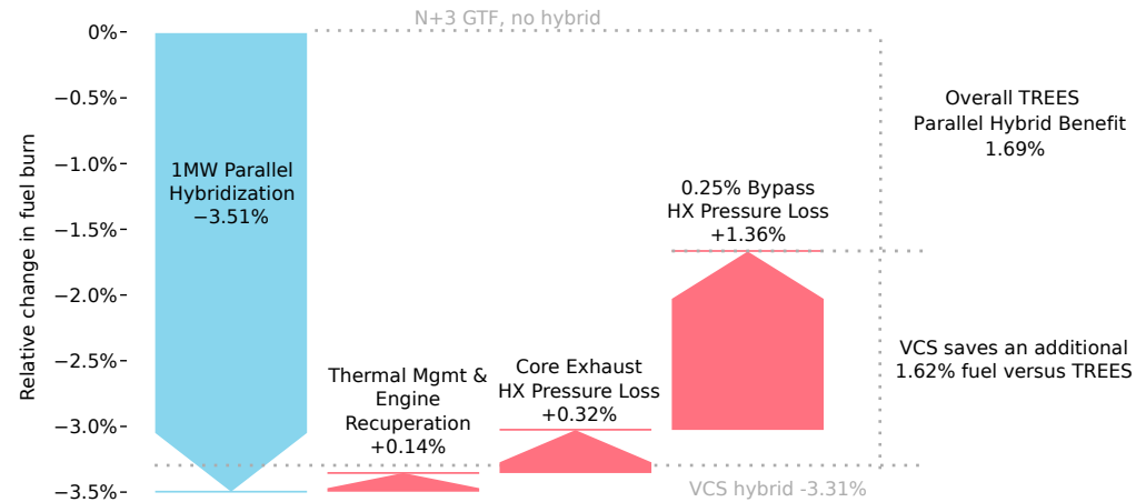
Figure 8. TREES has a smaller initial thermal management penalty due to the lighter cooling system and useful heat transfer to the turbofan's bypass. The total pressure losses from the heat exchangers in the turbofan's core and bypass negate this benefit.
