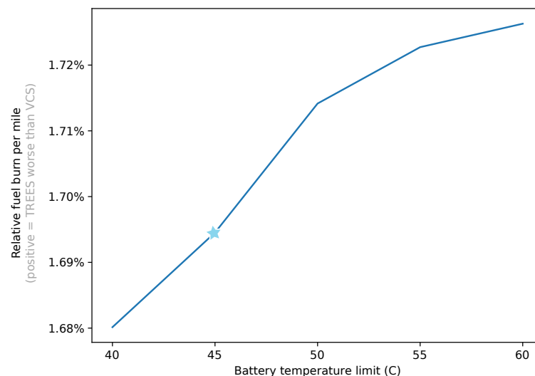
Figure 14. Increasing battery temperature limits favor the vapor cycle system because they allow a lighter chiller and smaller heat exchanger, whereas TREES can only shrink the heat exchanger, since the chiller is assumed to weigh nothing. The blue star marks the baseline battery temperature limit of 45 °C.
