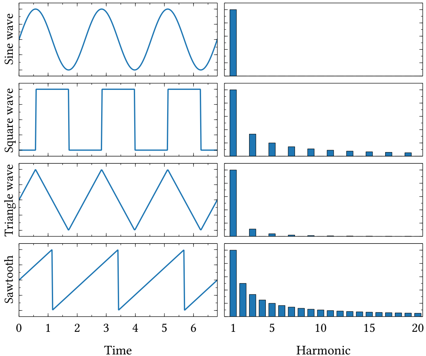
Waveform
