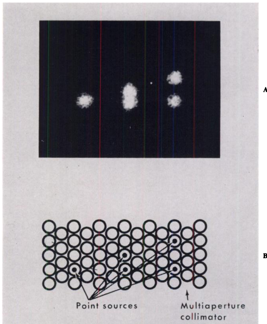
Fig. 4. Enlarged section of image showing 5 point sources of Ba^{133} resolved by the "A" multi-channel collimator. Sources are 1 inch from collimator and on the axes of holes shown in diagram.
