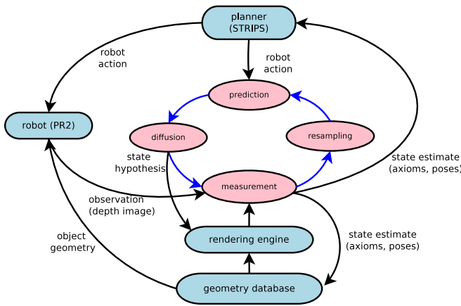
Fig. 4: System Architecture for sequential manipulation, with Axiomatic Particle Filter components highlighted.
