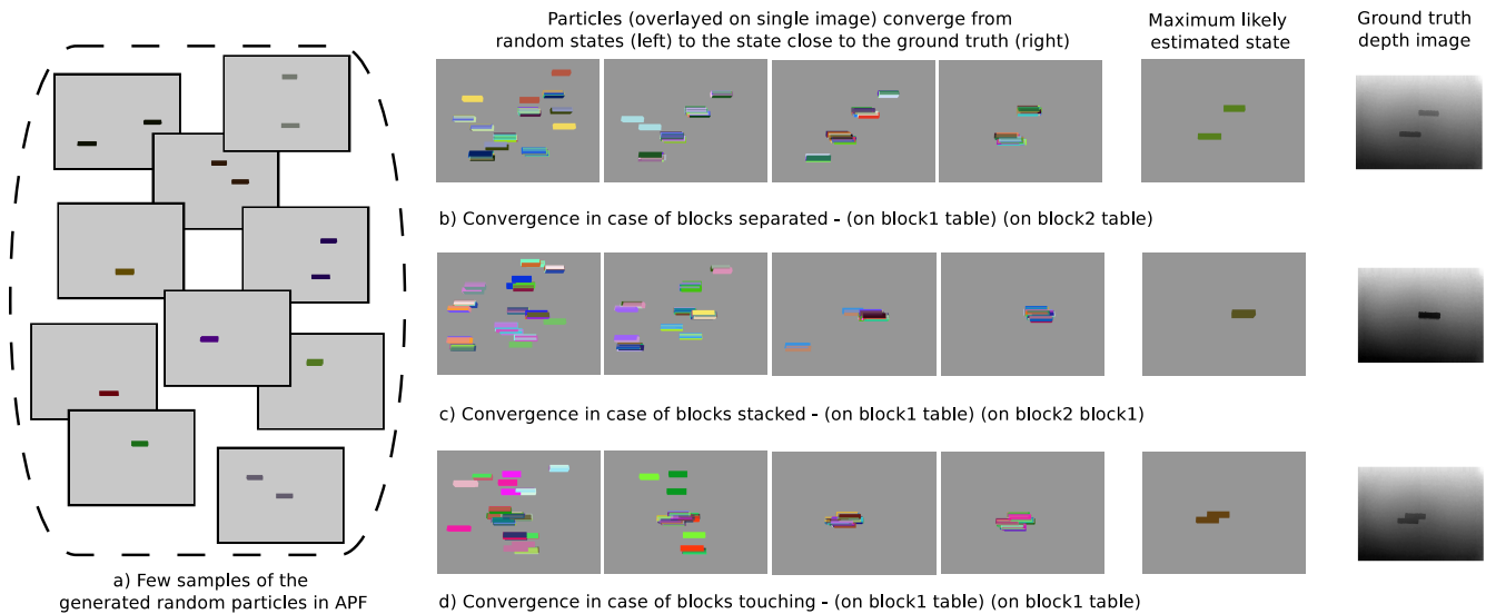
Fig. 6: Convergence of particles from the initial randomly generated states to the estimated state
