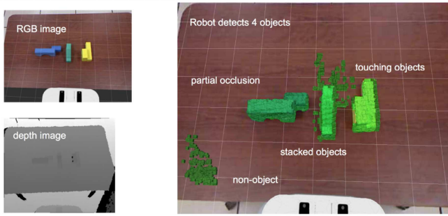
Fig. 2: Issues with object segmentation using the PR2 Interactive Manipulation [3]. Due to issues of uncertainty in open-loop perception, reliable autonomous robot manipulation is currently limited to distinctly separated objects on flat tabletops. For example, consider the scene of 6 simple blocks on a tabletop and its depth image from a Kinect RGBD camera on the head of a PR2 robot. The robot can find the tabletop, assuming it is the largest flat object in the scene. However, it cannot distinguish (and thus grasp directly) any of the individual objects due to occlusions, physical interaction, and false positives.
