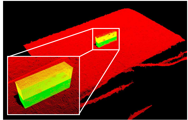
Fig. 5: Known geometries for the two stacked blocks example (yellow on green and green on a table) shown on the observed point cloud data.
